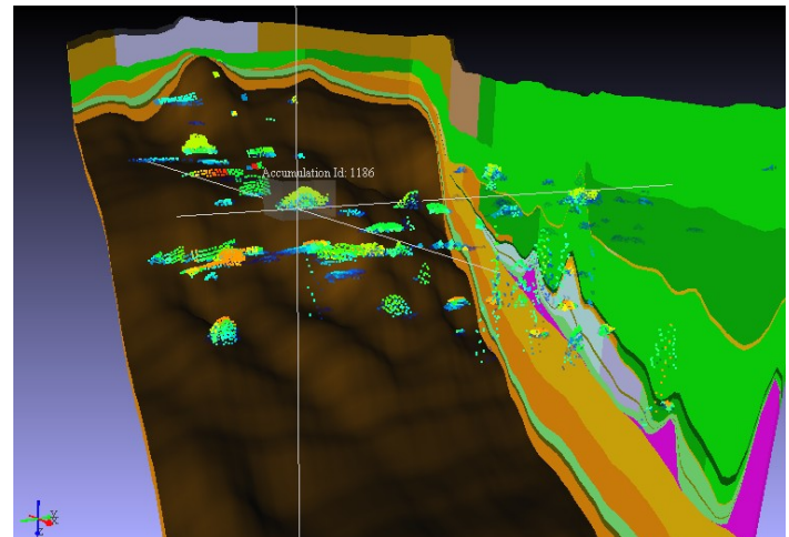
Simulation result highlighting fluid bodies of interest
